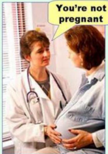
Type II error (false negative)
